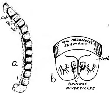
Fig. 225. a, Ptilodactyla serricollis Say; b, 9th and 10th abdominal segments.
